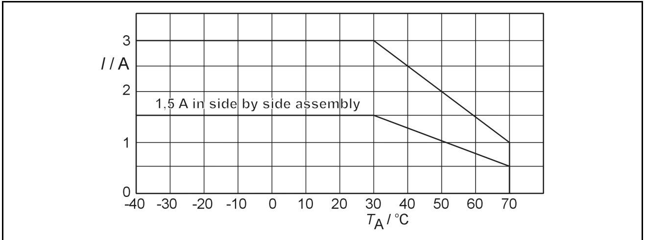
Derating curve for SLO 24CR.
